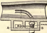
FIG. 2. INTERCEPTOR (DIVERTING).
